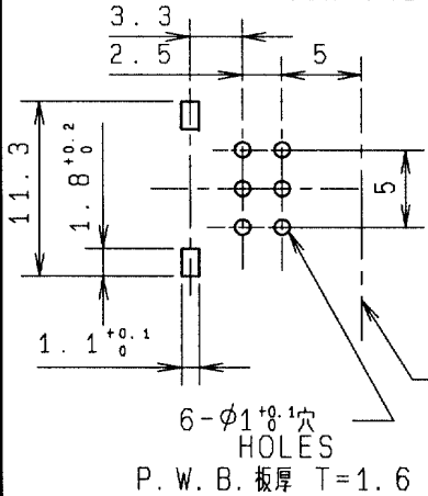
端子取付寸法図(挿入側より見を図) (許容差±0.1) MOUNTING HOLE DETAIL (TOLERANCE±0.1) VIEWED FROM MOUNTING SIDE
